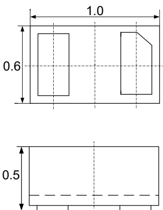
Package Dimensions
