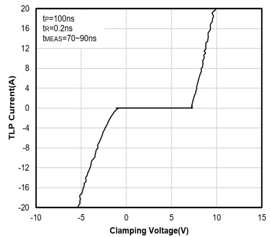
TLP Curve
